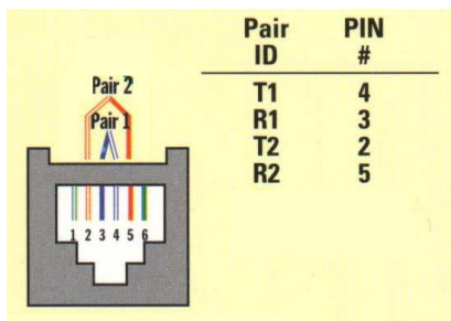
Figure 18 RJ11 & RJ14 POTS
