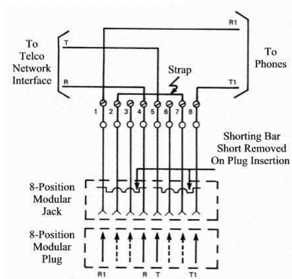
Figure 19 RJ31 & RJ38 Alarm Jack
