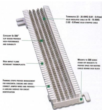
Figure 17 66-Block
