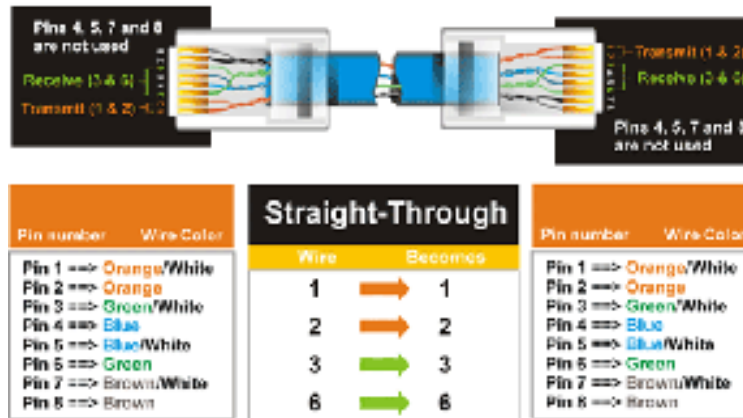
Figure 22 UTP Straight-through Patch Cable
