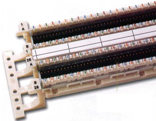
Figure 18 110-Block
