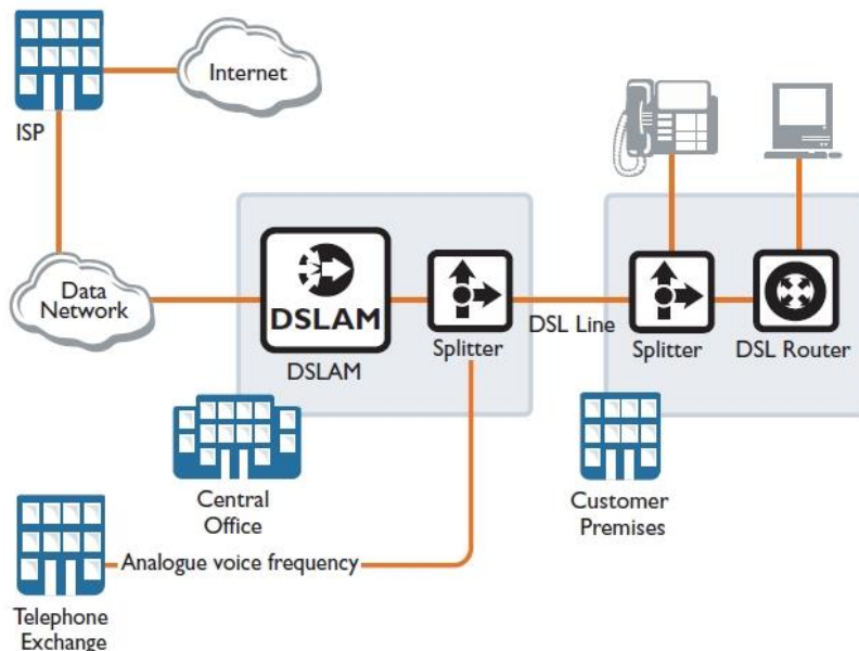
Figure 3 DSL Central Office to Customer
