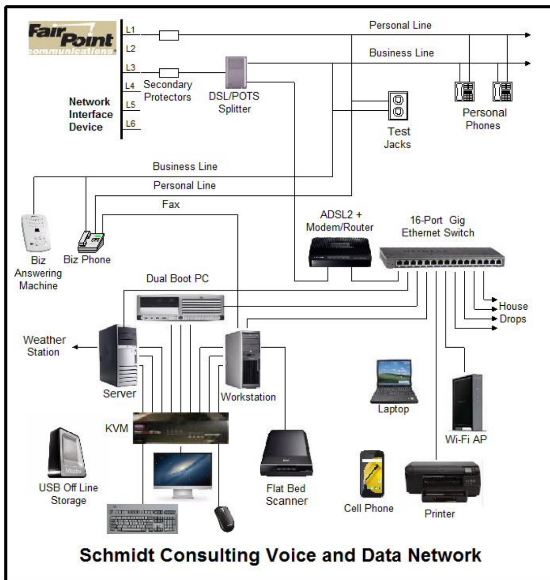
Figure 1 Schmidt Consulting Network
