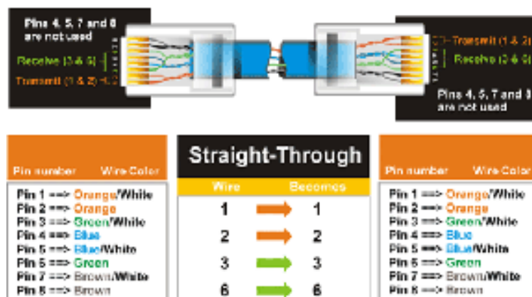
Figure 29 Patch Cable
