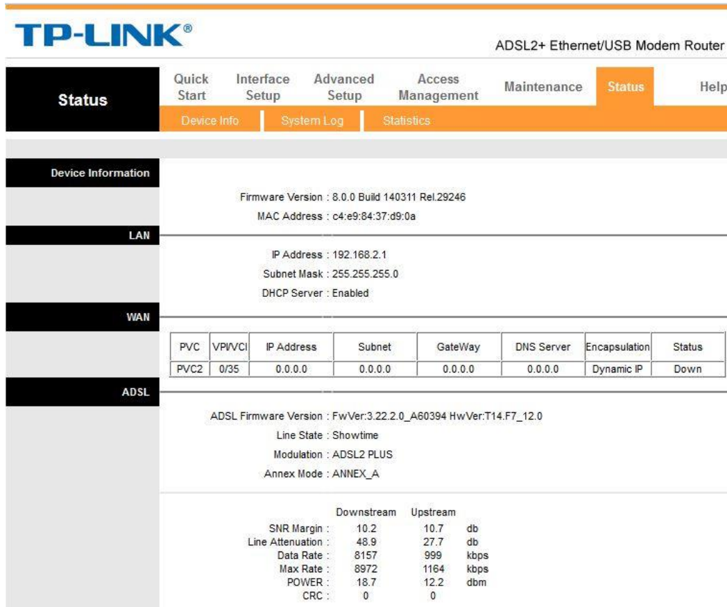
Figure 3 Router Status Page During DSL Initialization
