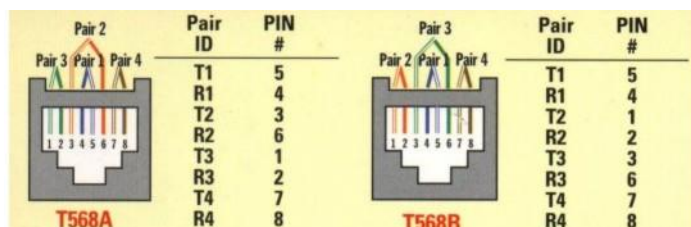
Figure 30 8P8C Structured Wiring Jacks
