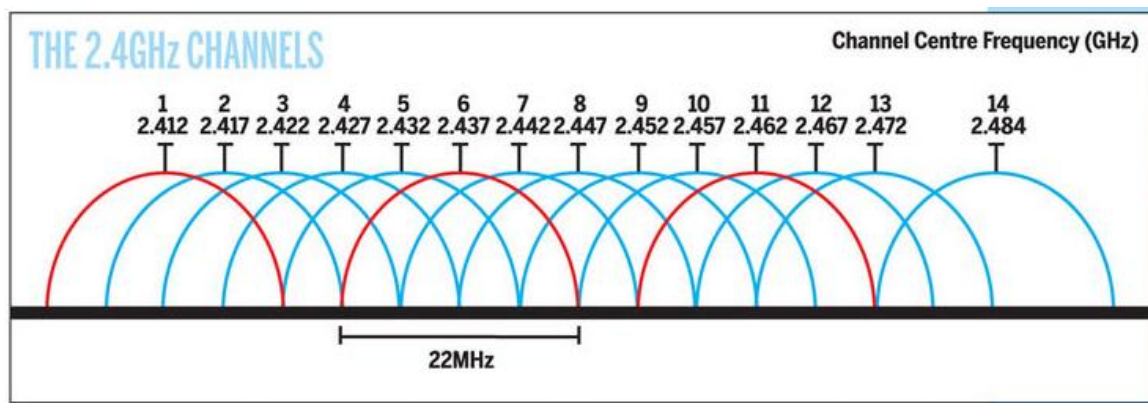
Figure 9 2.4GHz Wi-Fi Channels
