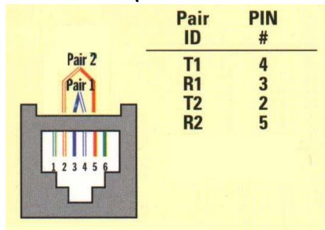
Figure 20 RJ11 & RJ14 Voice Jack
