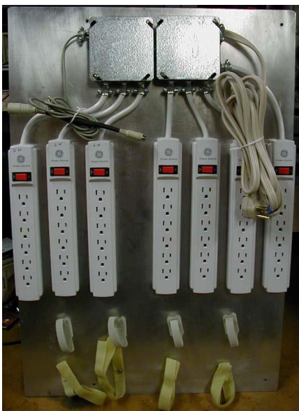
Figure 29 Power Distribution
