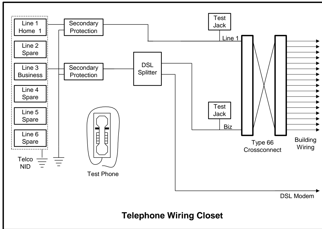
Figure 34 SOHO Telephone Wiring
