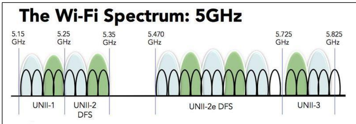
Figure 10 5GHz Wi-Fi Channels
