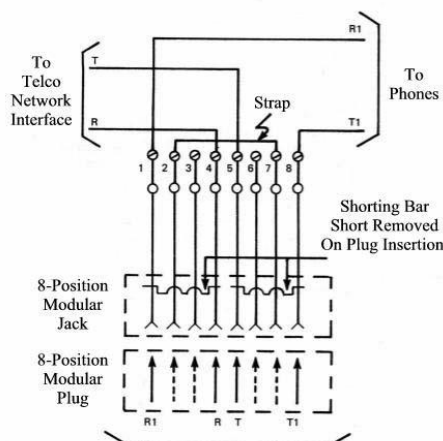
Figure 21 RJ38 Alarm Jack
